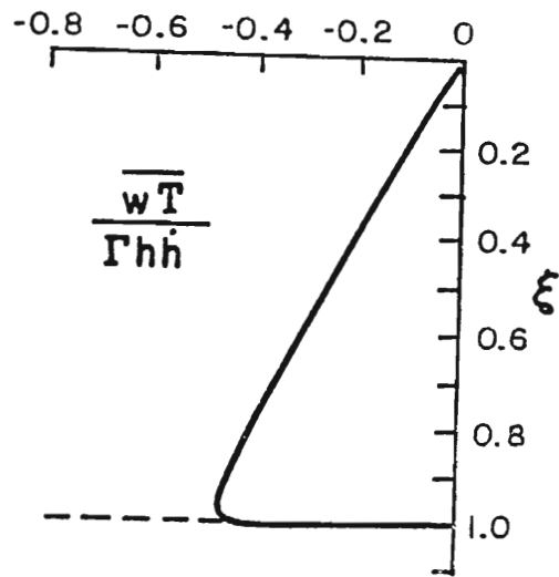
Figure 12. Profile of the vertical convective heat flux \overline{wT} , scaled by \Gamma h \dot{h} .
