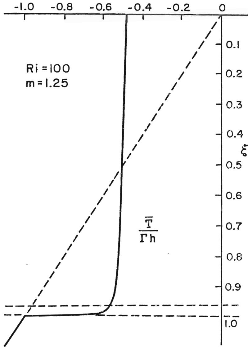
Figure 7. Mean temperature profile.
