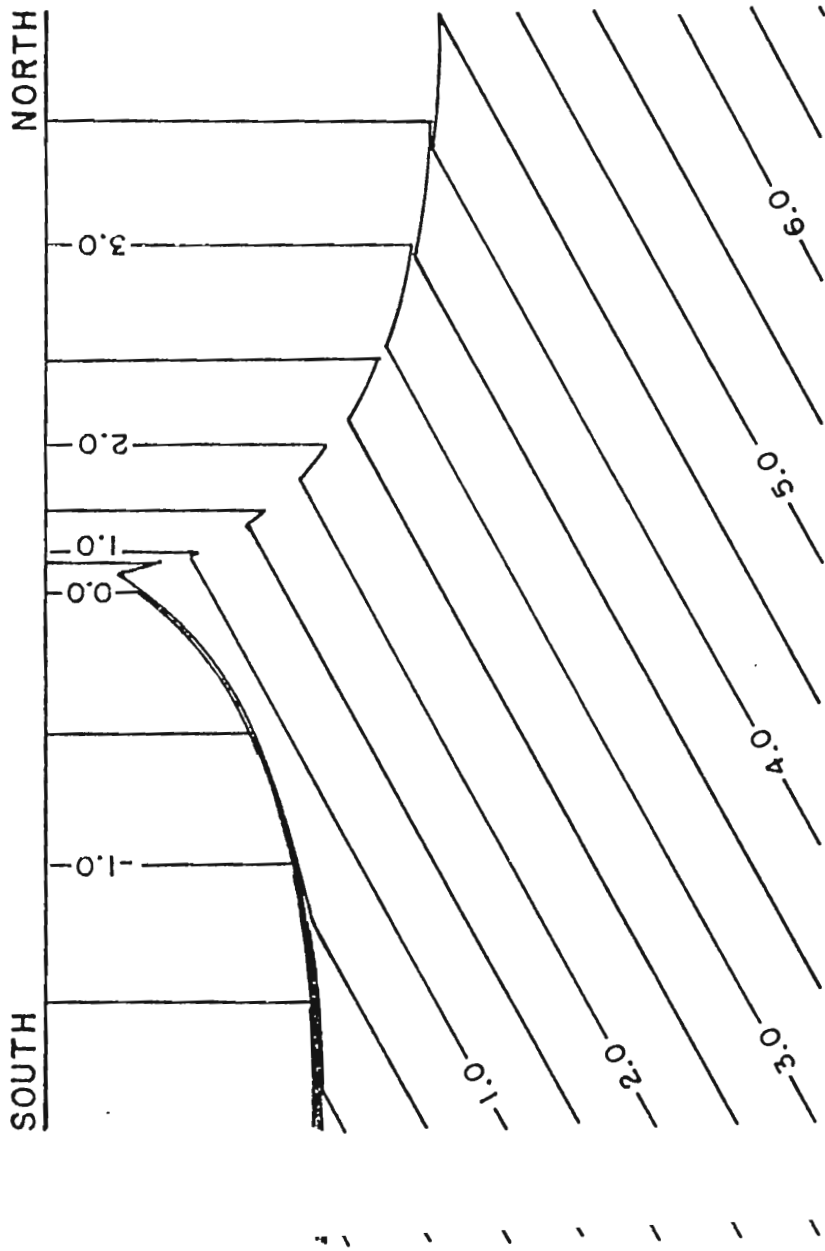
Figure 37. Cross-front section of the buoyancy field in the case of confluence, for t = 1.60 and a = 1.0 .
