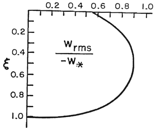
Figure 17. Vertical profile of the rms vertical velocity, scaled by -w_* .
