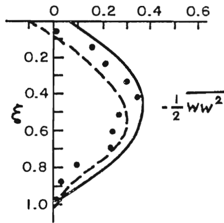
Figure 19. Vertical profiles of the vertical flux of turbulent kinetic energy, -\frac{1}{2} \overline{w w^2} , scaled by w_*^3 . The solid curve is the solution of the present model. The dashed curve is the numerical solution of Zeman and Lumley (1976). The dots represent the data of Willis and Deardorff (1974), run S1.
