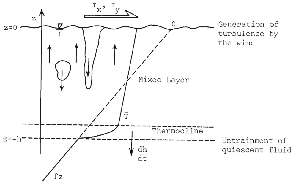
Figure 3. Schematic model of the wind-mixed layer.
