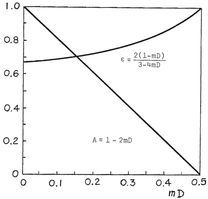
Figure 15. Plots of the coefficients \epsilon and A defined by (50) and (58); \epsilon is the ratio \bar{T}/(-\Gamma h) , and A is the ratio -(w\bar{T})_{-h}/Q .
