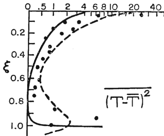
Figure 20. Vertical profiles of the temperature variance, \overline{(T - \bar{T})^2} , scaled by (u_0/Q)^2 . The solid curve is the solution of the present model. The dashed curve is the solution of Zeman and Lumley (1976). The dots represent the data of Willis and Deardorff (1974), run S1.
