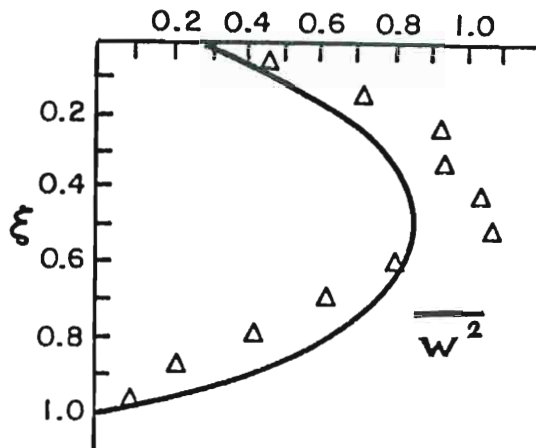
Figure 26. Vertical profile of the vertical-velocity variance, \overline{w^2} , scaled by w_0^2 , as on figure 18 but for Ri = 45 . The triangles represent the data of Willis and Deardorff (1974), run S2.
