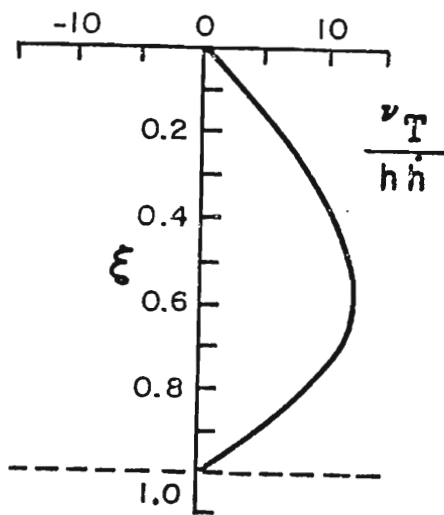
Figure 13. Profile of the eddy heat diffusivity \nu_T (cfr. text), scaled by h \dot{h} .
